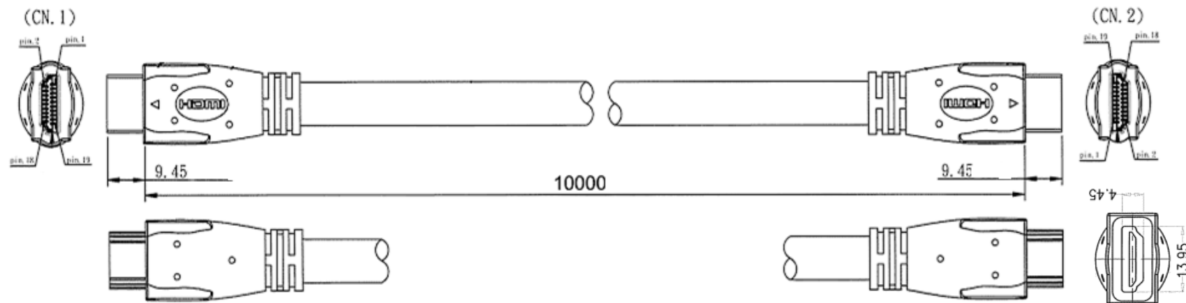
(A). Wire Pin Assignment and Wire Description.
