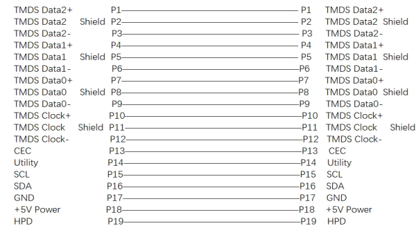
HDMI A Plug
