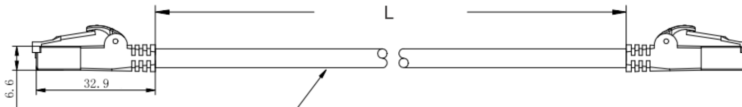
ELECOM Laned 24AWG/4P EIA/TIA-568-B.2-1 CAT.6 PATCH CABLE XXXXXXXXXX A
